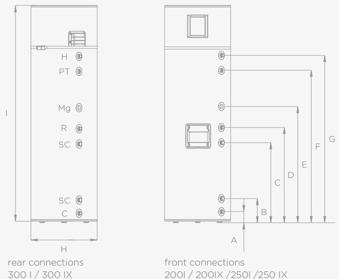
Equipment: Storage Water Heater
