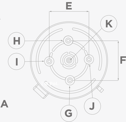
THERMOCYLINDER | CONEXIONES STANDARD
